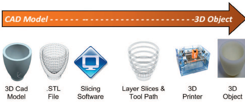
Figure 19. The 3D Printing process [79]
