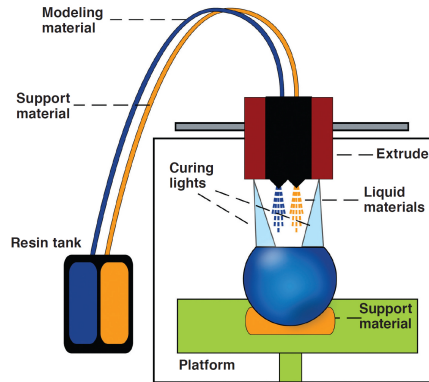
Figure 21. Representation of PolyJet photopolymer (PPP) 3D printing [77]
